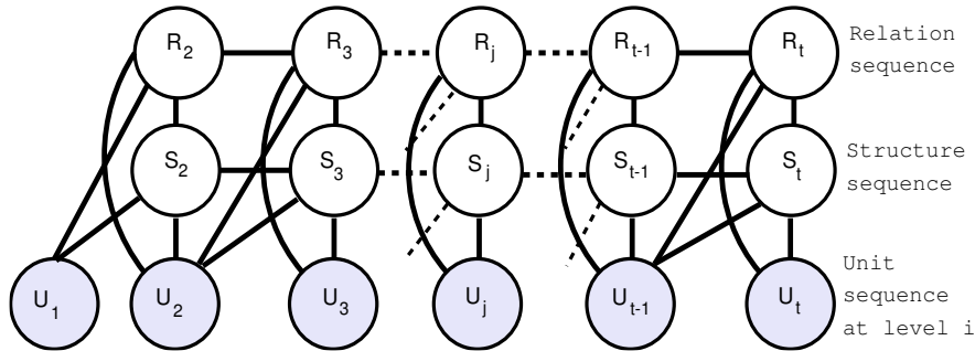
Figure 5: The intra-sentential parsing model of CODRA.
