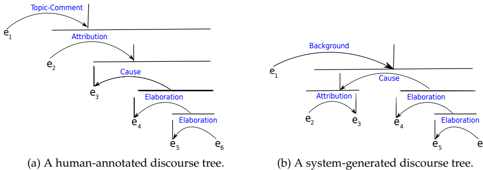
Figure 17: Discourse trees generated by human annotator and our system for the text [what’s more,]e1 [he believes]e2 [seasonal swings in the auto industry this year aren’t occurring at the same time in the past,]e3 [because of production and pricing differences]e4 [that are curbing the accuracy of seasonal adjustments]e5 [built into the employment data.]e6
