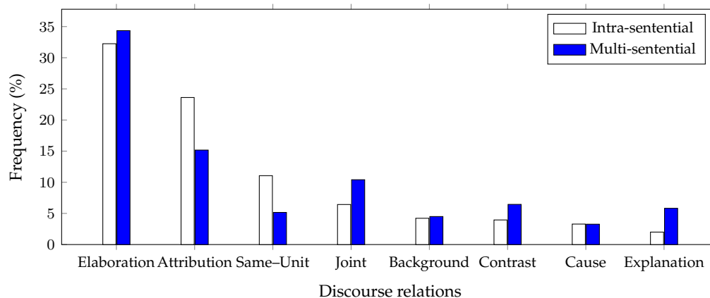
Figure 3: Distributions of eight most frequent relations in intra-sentential and multi-sentential parsing scenarios on the RST-DT training set.
